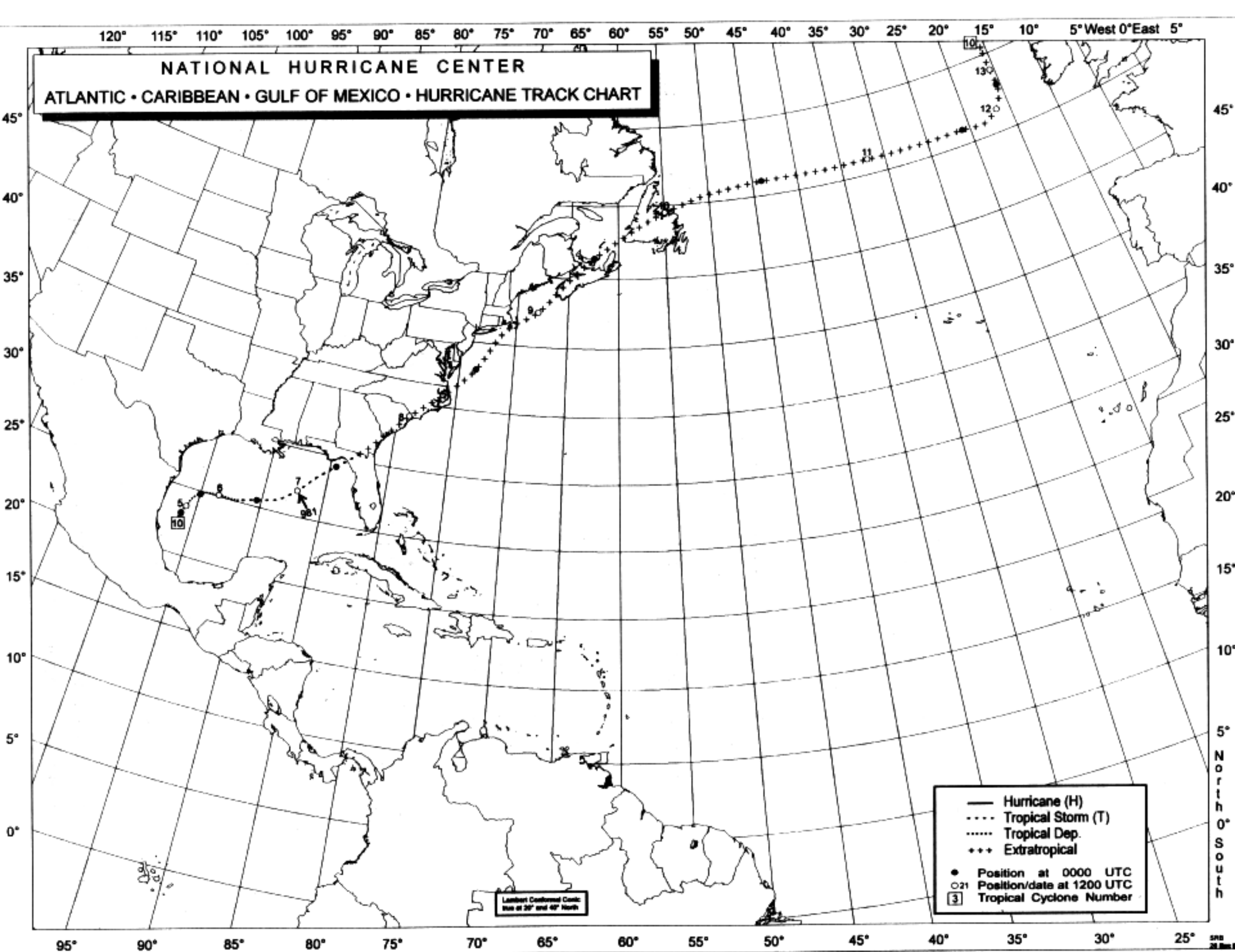
Figure 1. Best track positions for Tropical Storm Josephine, October, 1996
