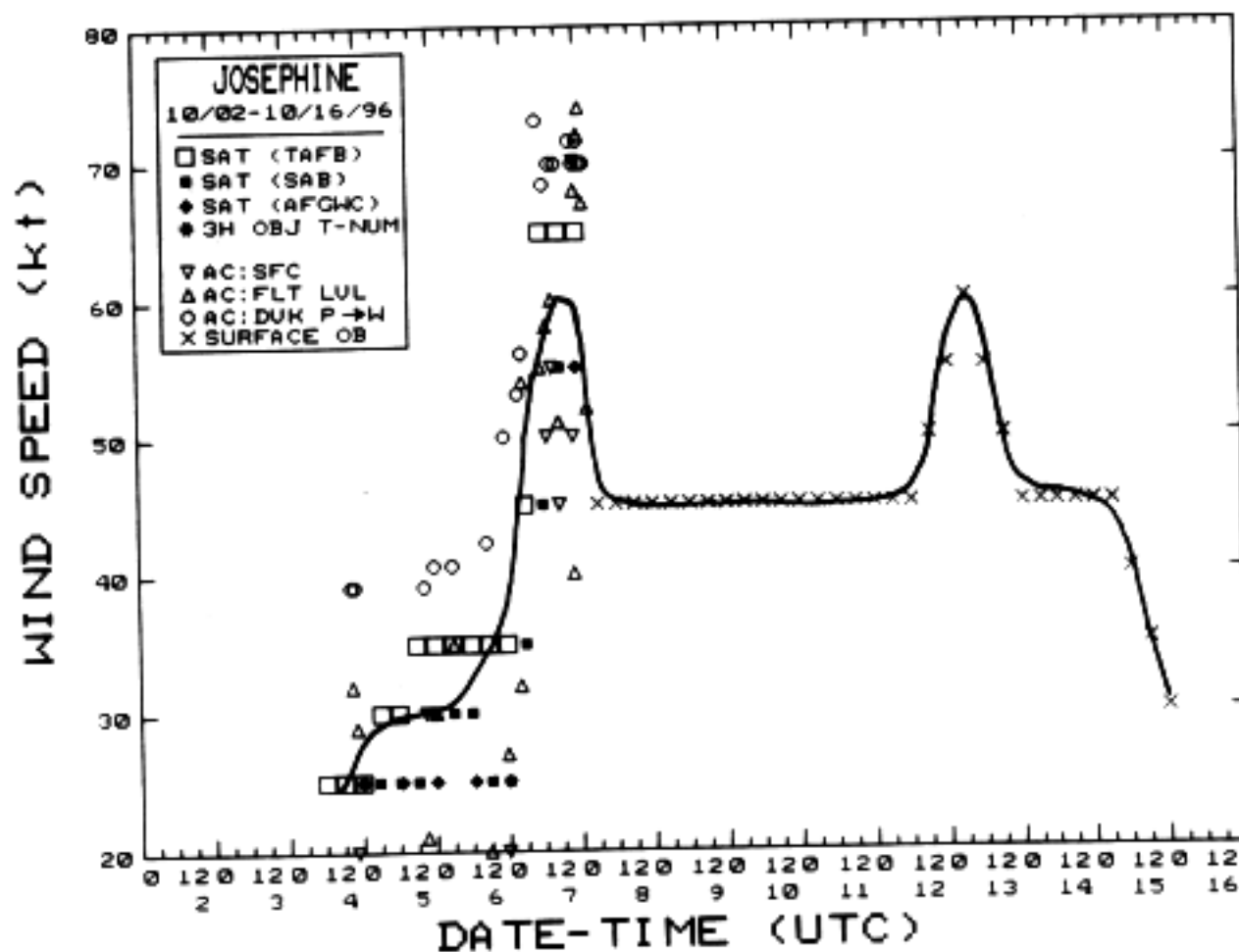
Figure 3. Best track maximum one-minute wind speed curve for Tropical Storm Josephine, October, 1996.
