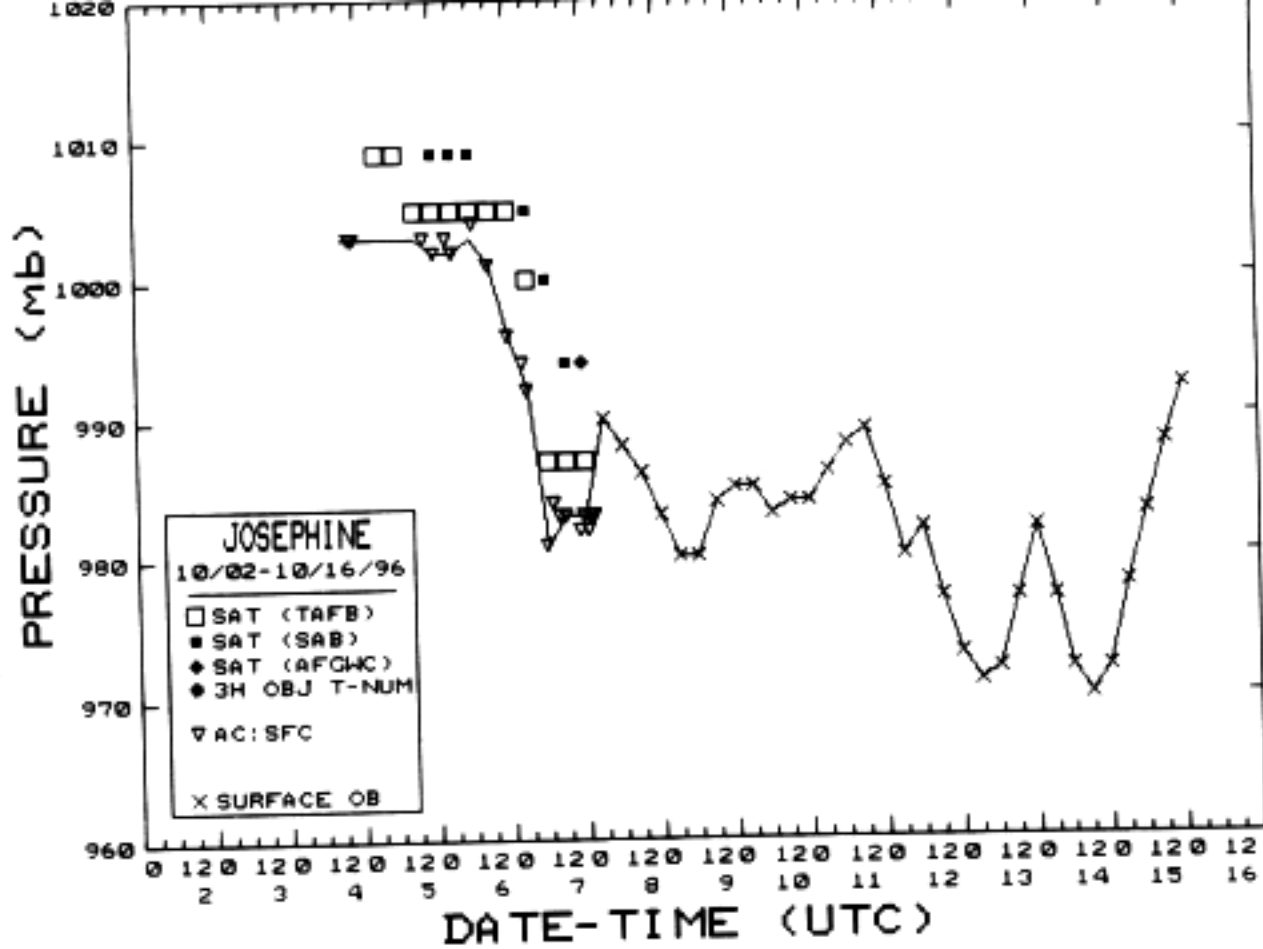
Figure 2. Best track minimum central pressure curve for Tropical Storm Josephine, October, 1996.
