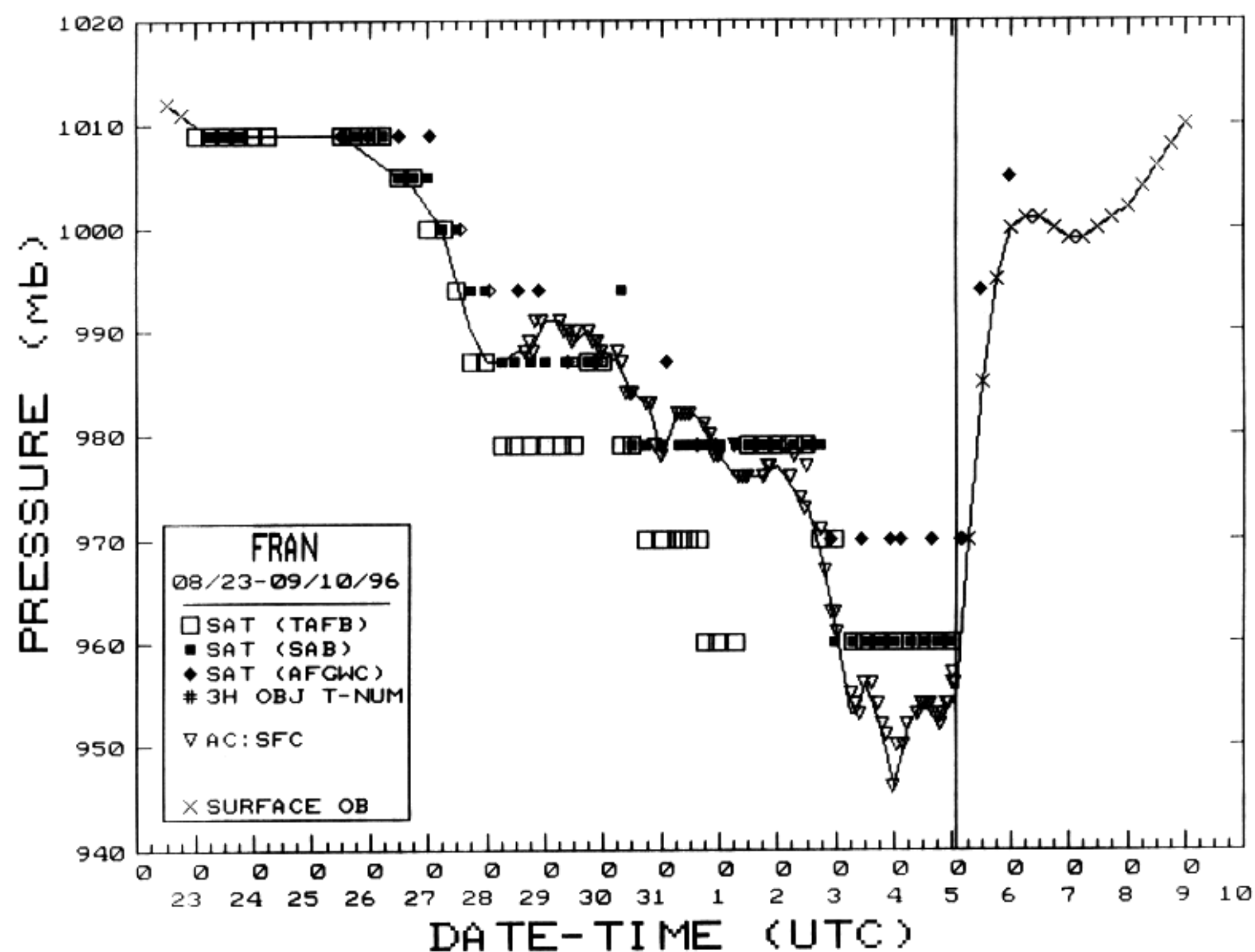
Figure 2. Best track minimum central pressure curve for Hurricane Fran. Vertical line denotes landfall. X's indicate estimates from surface analyses.
