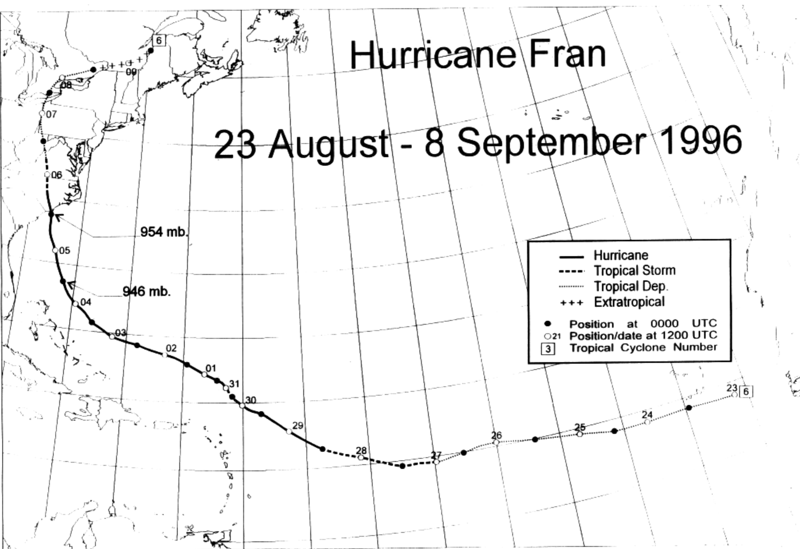
Figure 1. Best track positions for Hurricane Fran, 23 August - 8 September 1996.
