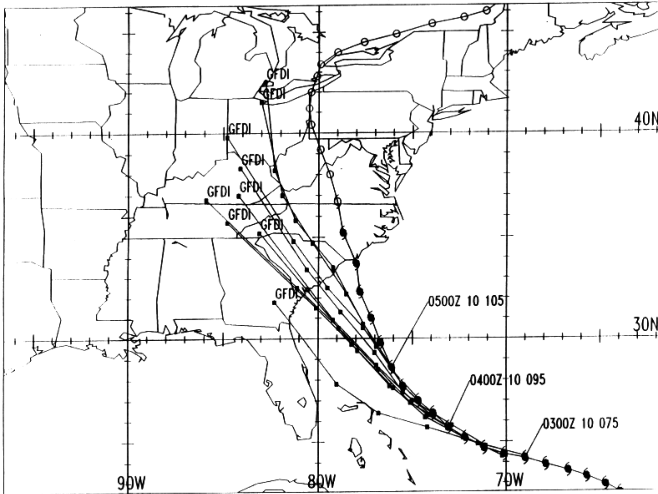
Figure 4. GFDL guidance on Hurricane Fran from 0000 UTC 3 September to 0000 UTC 5 September showing a left bias.
