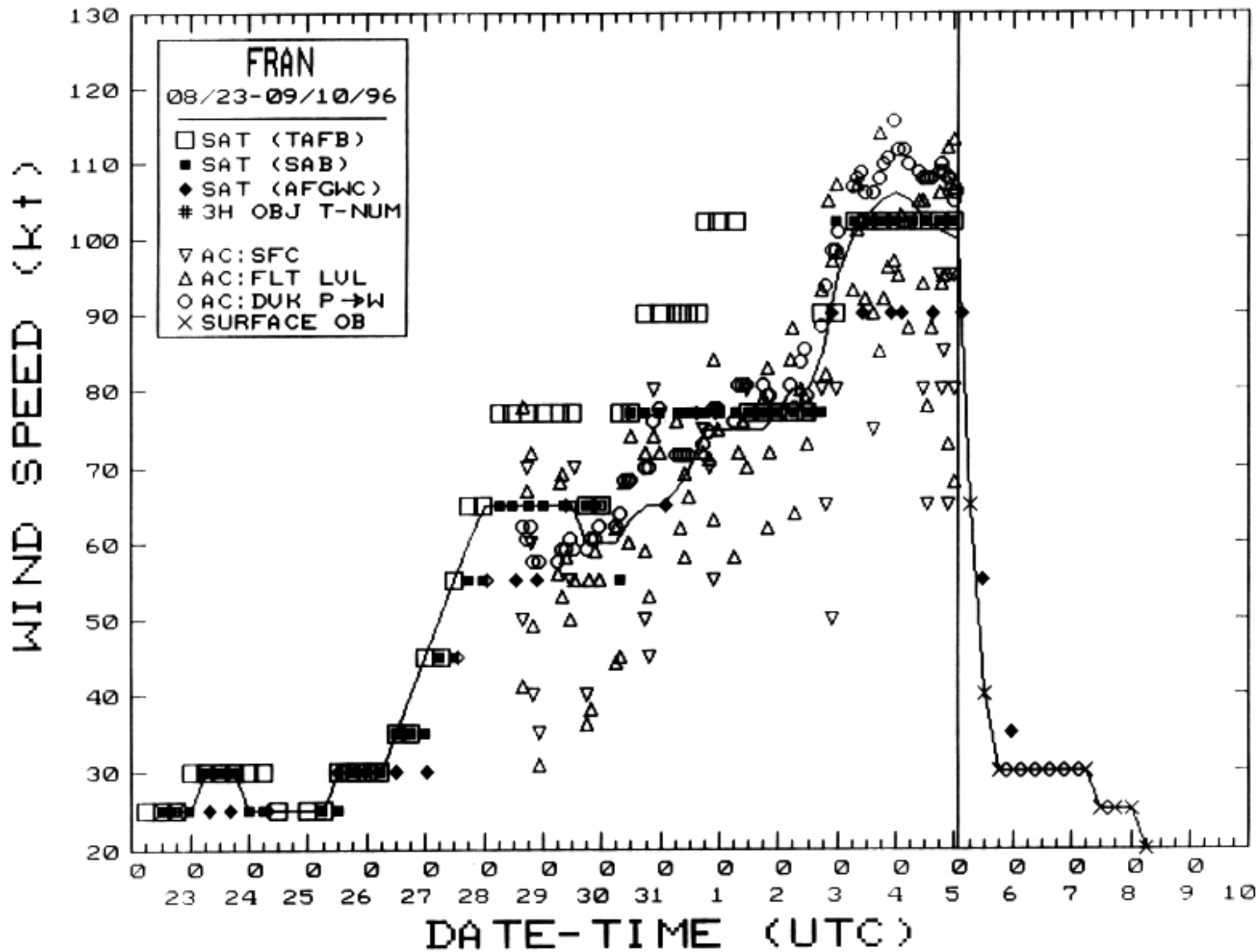
Figure 3. Best track maximum sustained wind speed curve for Hurricane Fran. Vertical line denotes landfall. Not all aircraft observations are a sampling of the maximum wind. X's indicate estimates from surface analyses.
