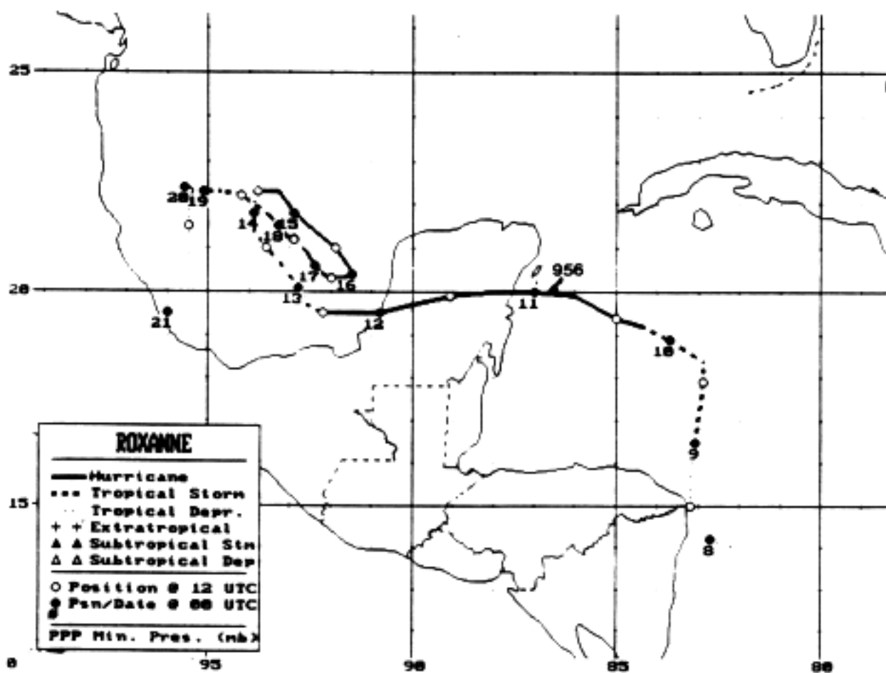
Fig. 3. Best track positions for Hurricane Roxanne, 7-21 October 1995.
